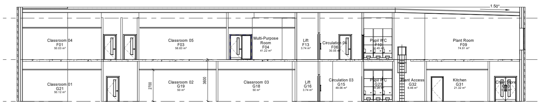
Section 04 through teaching wing
