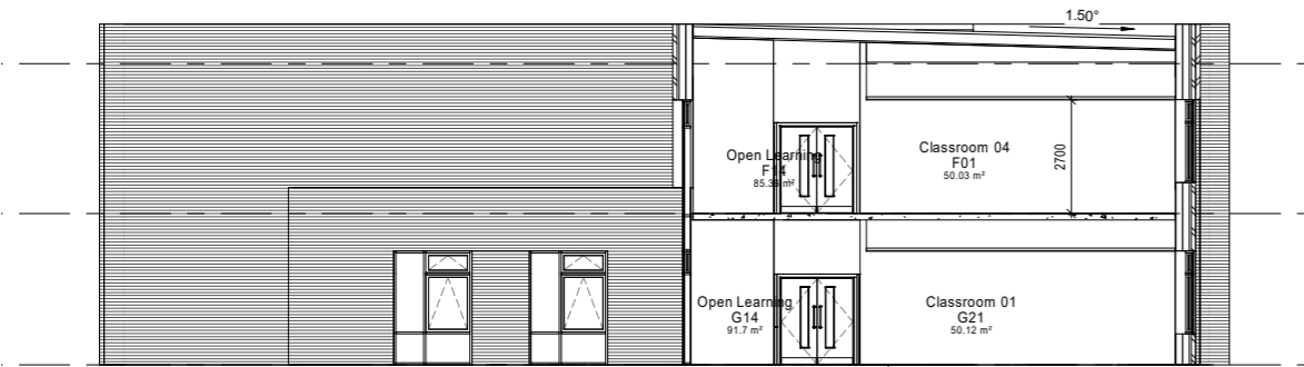
Section 01 through teaching wing
