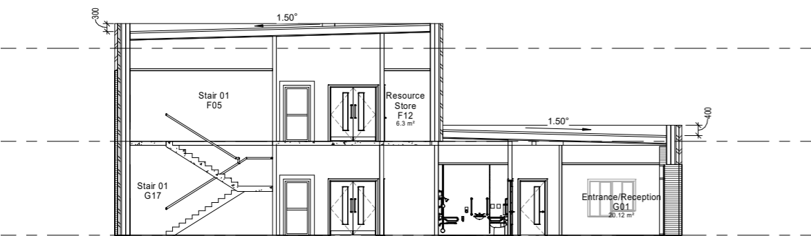
Section 03 through circulation
